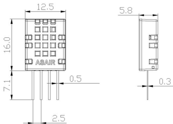
Figure 5. AGS02MA dimensions (unit: mm, general tolerances: ISO2768-mK)
