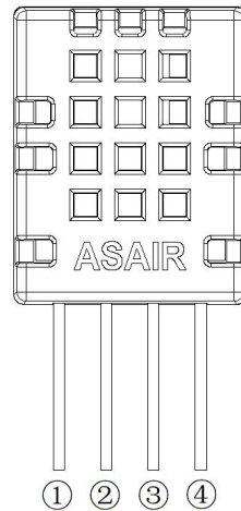
Figure 4. AGS02MA pinout
